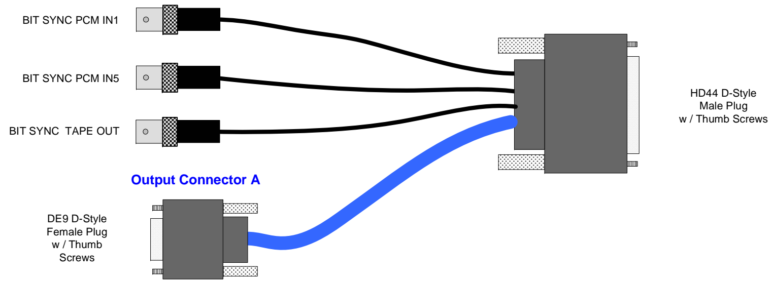
Output Connector A Connection Table
