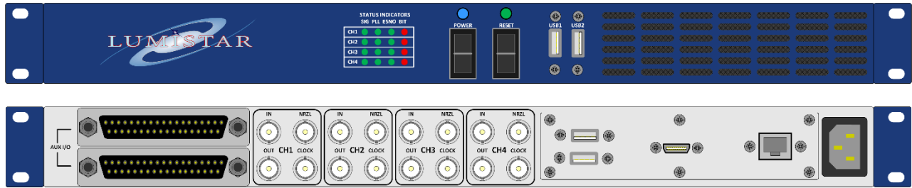
LS-45-R1P-QBS Front and Rear Panel Elevations (Quad Version Shown)
